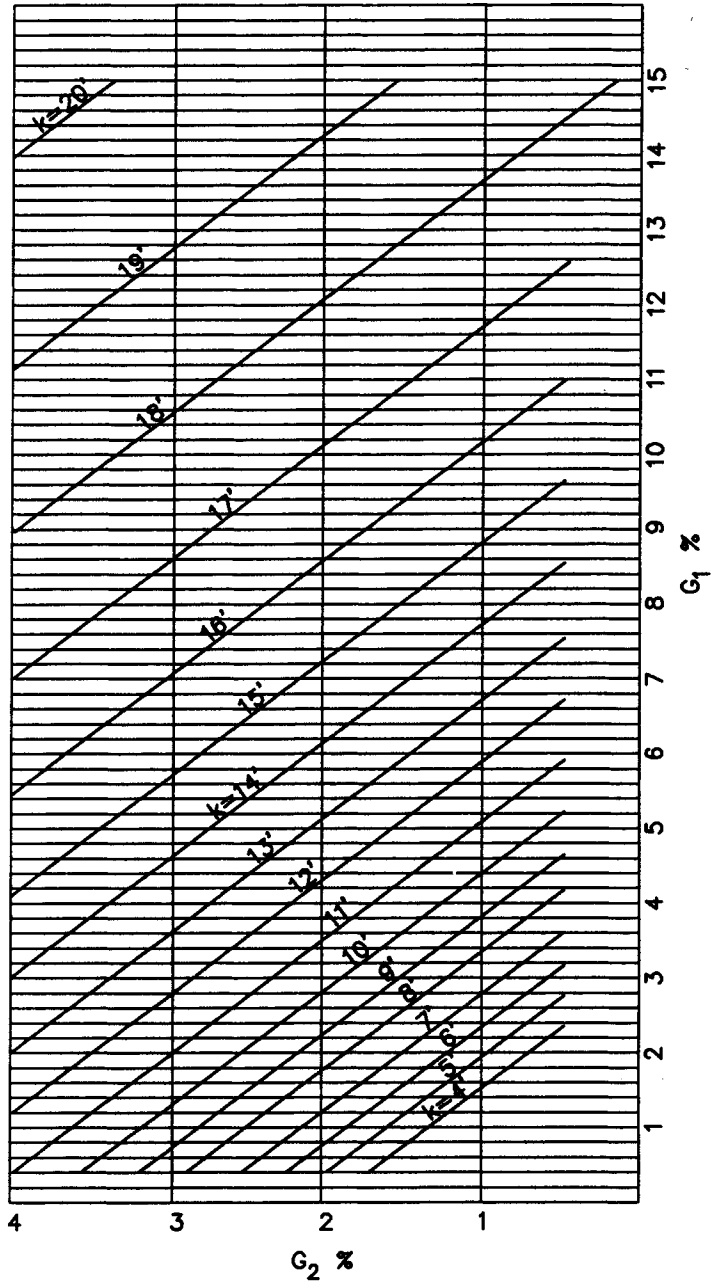
GRAPH USED TO DETERMINE "K" ONLY
