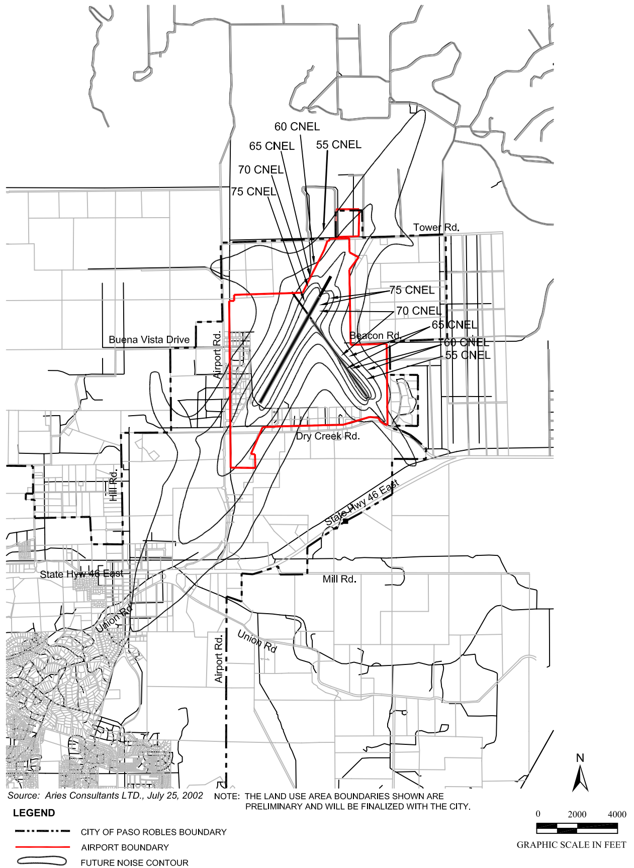
Future Airport Noise Contours (2020)
